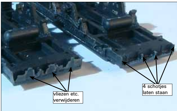
Foto 7: Schoonmaken bufferbalk
